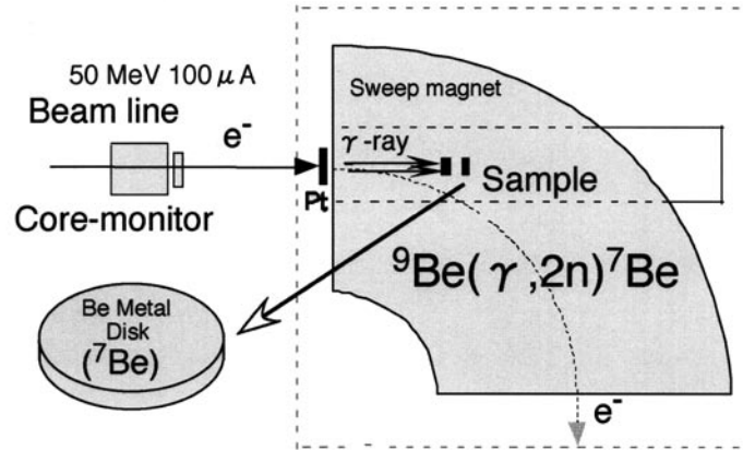
Fig.1. Setup for irradiation of Be metal.
