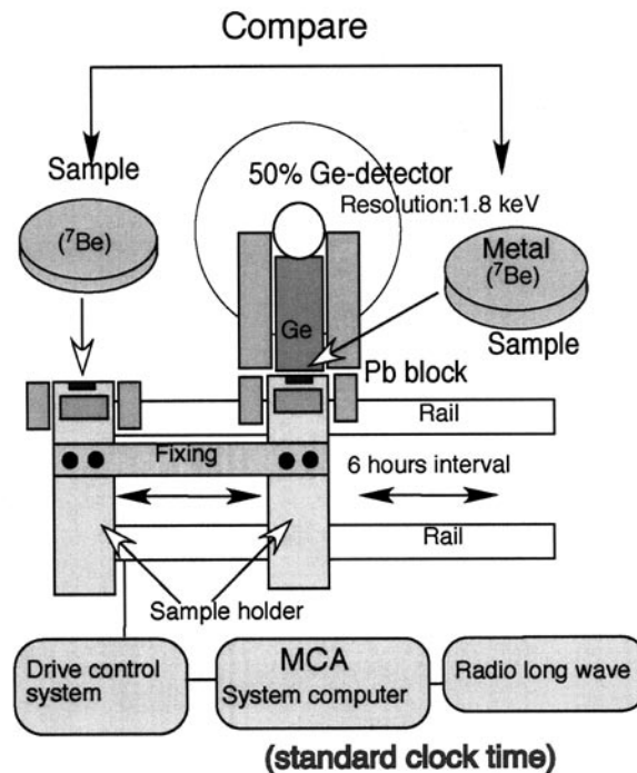
Fig.2. Experimental setup.
