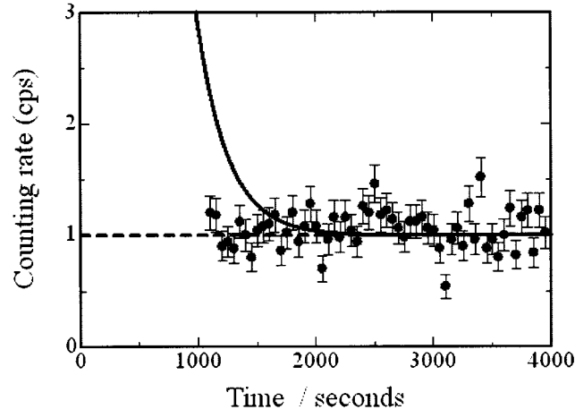
Fig.1. Time variation of the counting rate for photons emitted from ^{229\text{m}}\text{Th} \text{HNO}_3 solution sample grown for 2 hours in the 9M HCl.
