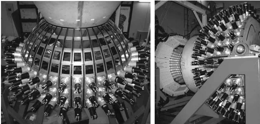
Fig.2. LEPS Backward Gamma. The left panel shows a photo of the LEPS Backward Gamma when the 90^\circ – 100^\circ , 80^\circ – 90^\circ , and 70^\circ – 80^\circ Lead/SciFi modules were stacked. The right panel shows a photo of the constructed Backward Gamma together with SCISSORS III.
