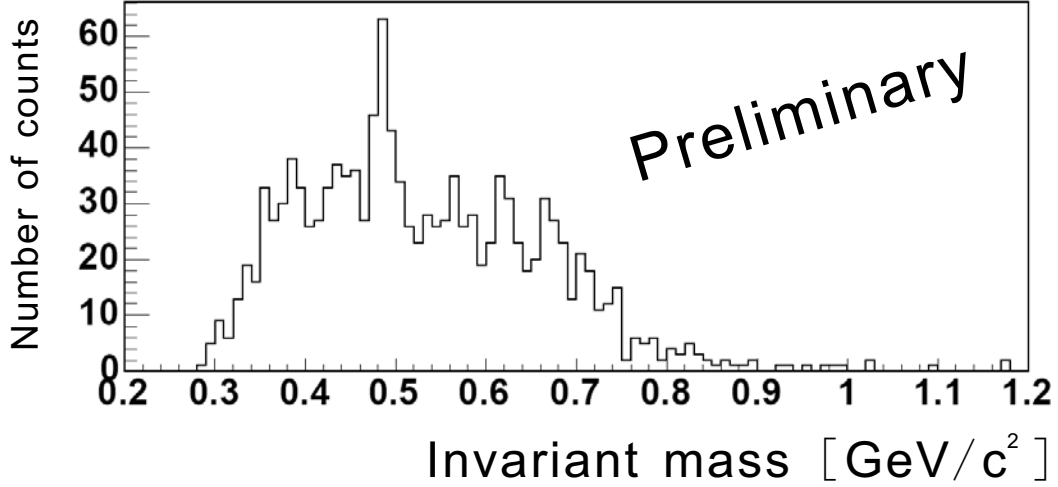
Fig.5. The invariant mass distribution of \pi^+\pi^- pairs in 0.8 < E_\gamma < 1.1 GeV.
